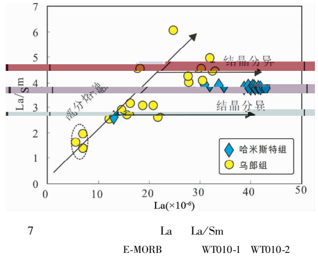
7 La La/Sm E-MORB OIB Sr-Nd WT010-1 WT010-2 WT012-1 Fig. 7 La vs. La/Sm of the Nileke Permian volcanic rocks
